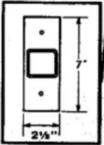
Base Plate
