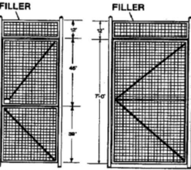
DUTCH DOOR SWING GATE
