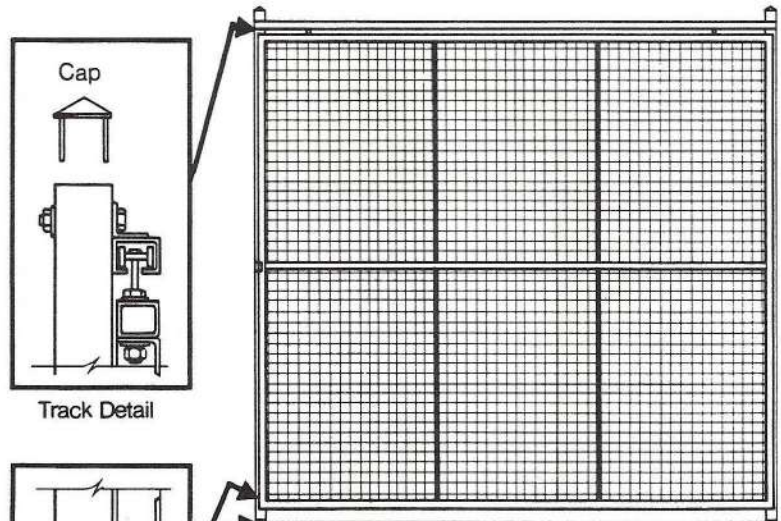
SLIDING GATE
