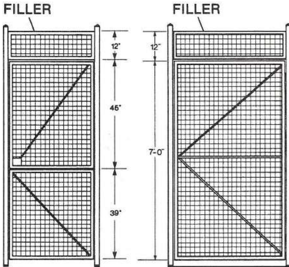
DUTCH DOOR
