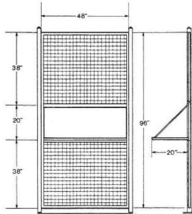
SERVICE WICKET
